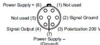
7-pin LEMO plug 1B male (ext. view)
