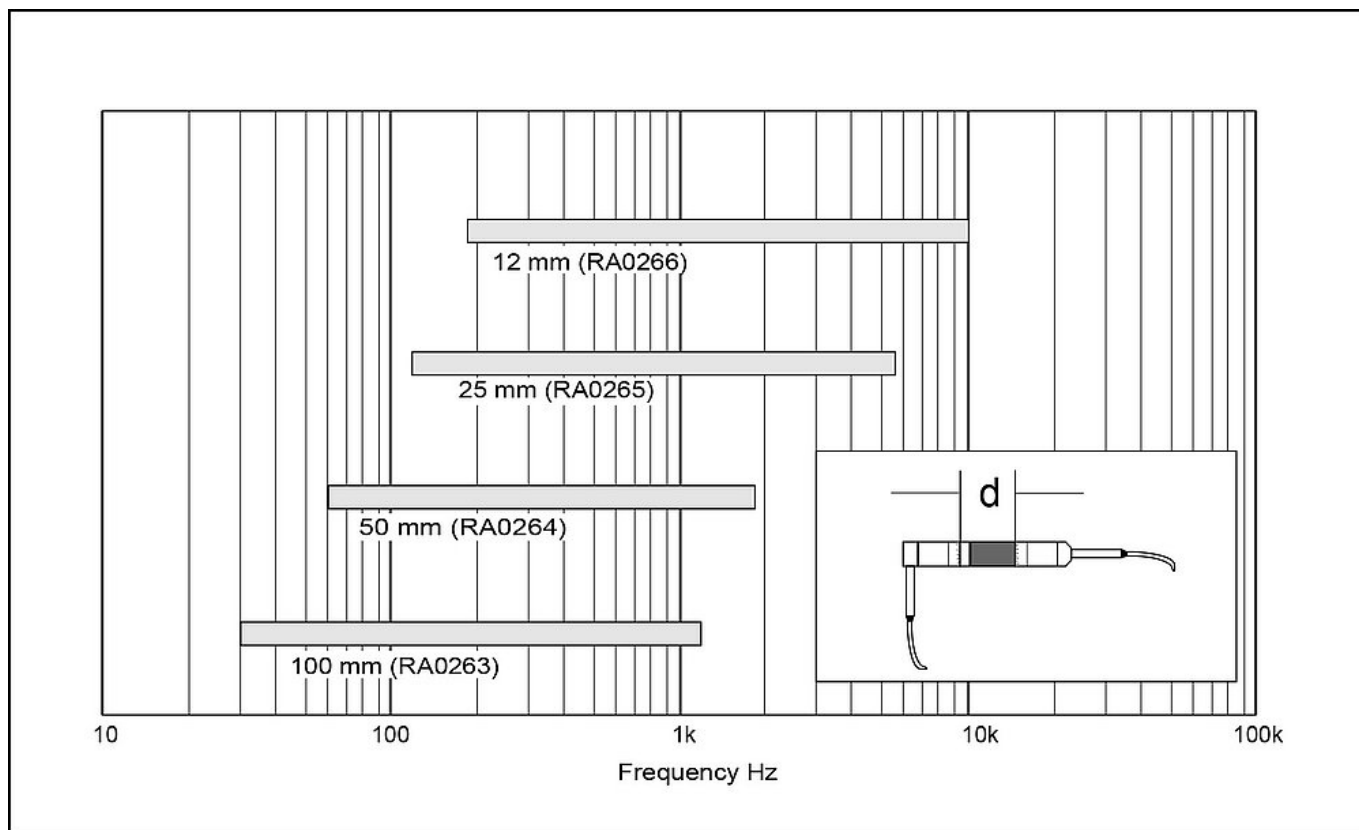
Frequency ranges for different microphone spacers
