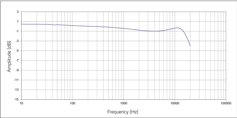
Typical pressure frequency response
